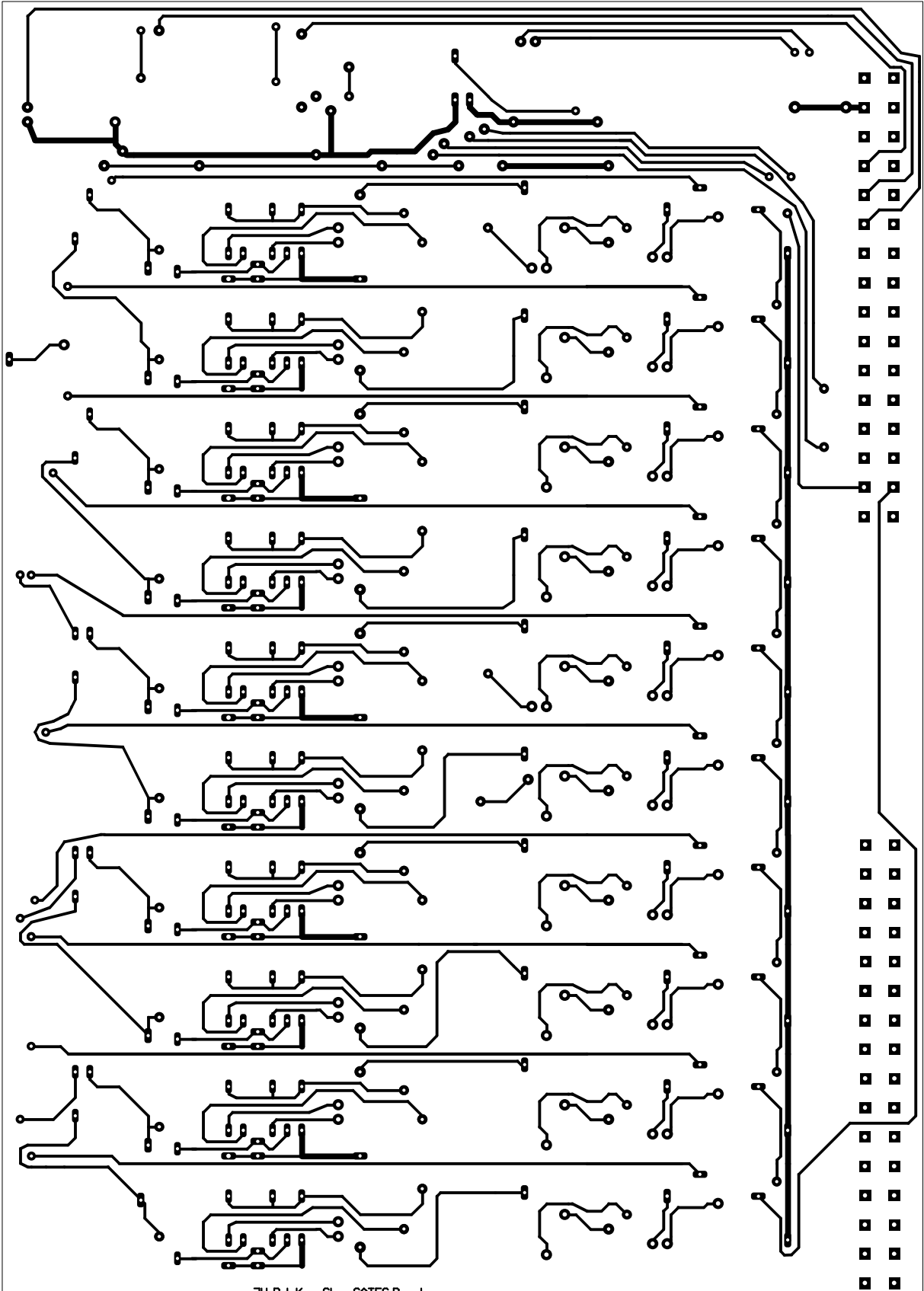
JH. Pol-Korg Clone GATES Board (c) J. Haible 2002
